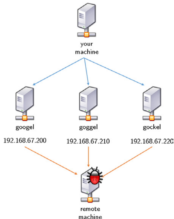
Figure 2: Covert channel through unaware servers.
